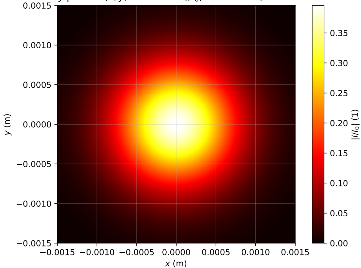
Intensity profile I(x, y, z = 3.503m)/I_0 , P_{in}=0.4P_{cr} , artificial time
